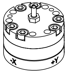
MINI27TI-A ISOMETRIC VIEW
